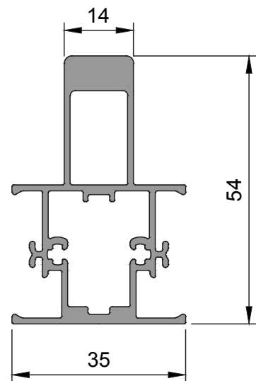
Evolution Mullion 54 mm W58362
