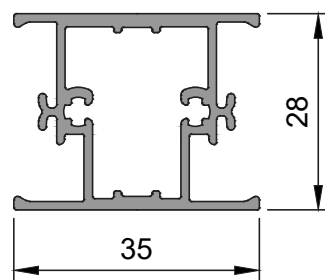
Evolution Mullion 28 mm W58086
