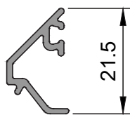
Evolution Bevel Bead 13 mm Gap W36274
