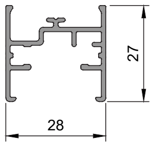
Evolution Frame W36276
