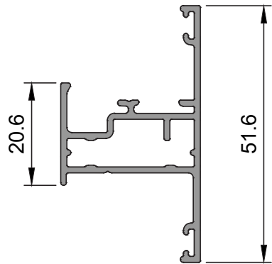
Evolution Sash Bottom Hung W58087
