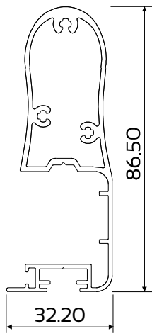
DIE No. W54318 Heavy Duty Interlocker
