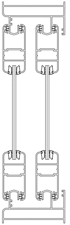
SECTION B-B Section not to scale
