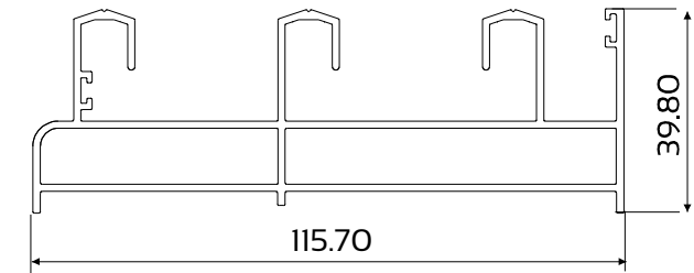
DIE No. W54299 Triple Frame with Lip
