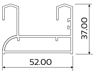
DIE No. *W50827 Outer Frame Double Track
