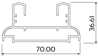
DIE No. *W50879 Symmetrical Double Track
