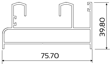
DIE No. W54272 Outer Frame with Lip
