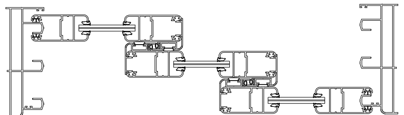
SECTION A-A Section not to scale
