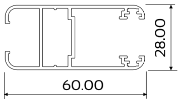
DIE No. W50855 Sash Frame
