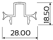
DIE No. W72183 Astragal for Meeting Stile
