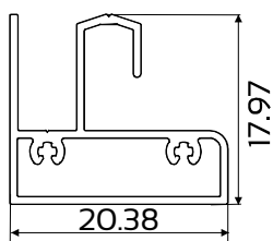
DIE No. *W54400 Outer Frame Shutter
