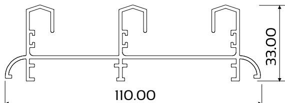
DIE No. *W29233 Frame 44mm Flat
