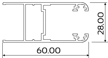
DIE No. W54274 Heavy Duty Sash Frame
