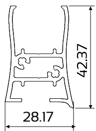
DIE No. *W54022 Heavy Duty Handle
