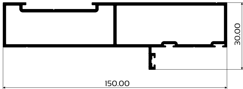
DIE No. W57566 Horizon Jamb Rail
