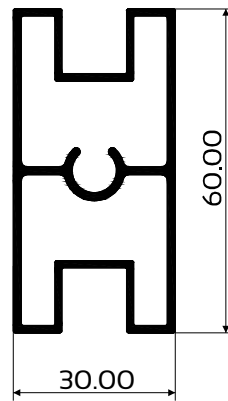
DIE No. W56086 Midrail 32mm
