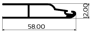
DIE No. W55469 Top/Bottom Louvre
