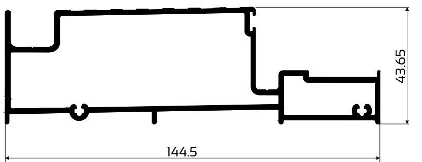
DIE No. W57568 Horizon Sill Rail
