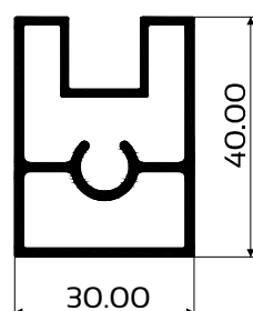
DIE No. W56085 Top/Bottom 32mm
