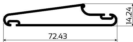
DIE No. W55474 Adjustable Louvre
