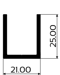
DIE No. W26152 U-Channel
