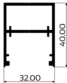
DIE No. W56087 Stile 32mm
