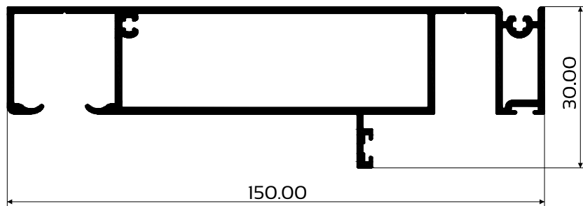
DIE No. W57567 Horizon Head Rail
