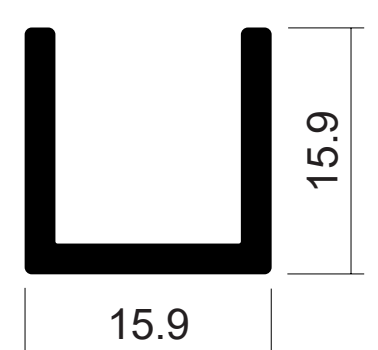
DIE No. W20042 | U-channel 15.9 x 15.9 x 1.7
