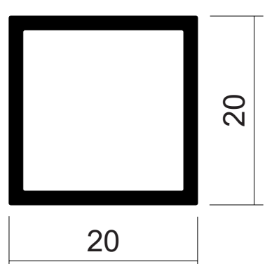
DIE No. W42179 | Square Tube 20 x 20 x 1.5
