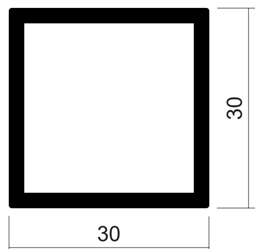
DIE No. W42886 | Square Tube 30 x 30 x 2
