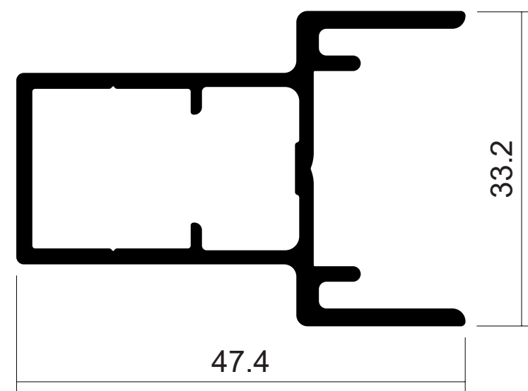
DIE No. W59150 | Guardian Lock Stile
