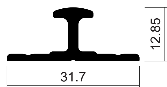
DIE No. W37997 | Guardian Track
