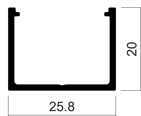
DIE No. W38002 | U-channel 25.8 x 20 x 1.5
