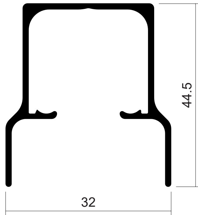
DIE No. W38001 | Guardian Head Rail
