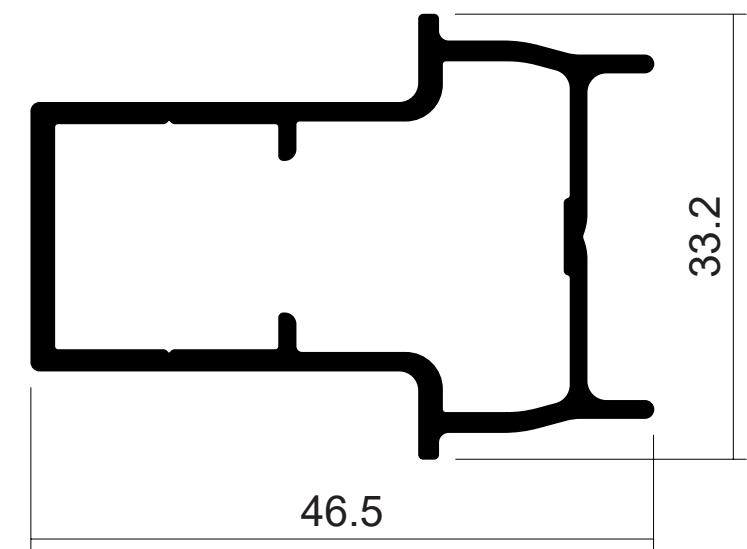
DIE No. W59152 | Guardian Meeting Stile
