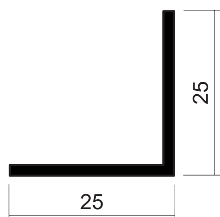
DIE No. W10968 | Eq. Angle 25 x 25 x 1.6
