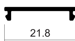
DIE No. W32321 | Guardian Clip-on Cover
