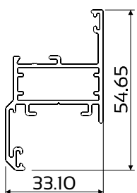
DIE No. W57602 Swift 30.5 Sash Euro
