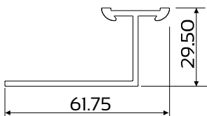
DIE No. W28002 Swift 30.5 Fixing Lug Twist In
