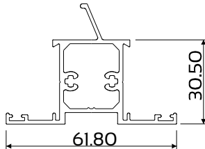
DIE No. W53630 Swift 30.5 Mullion 30mm Weather Bar
