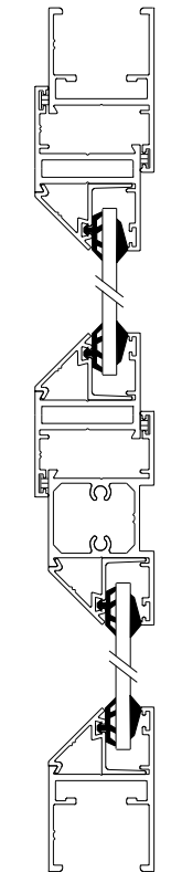
SECTION B-B Section not to scale
