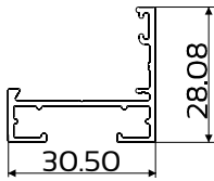
DIE No. W36831 Swift 30.5 Short Leg Frame
