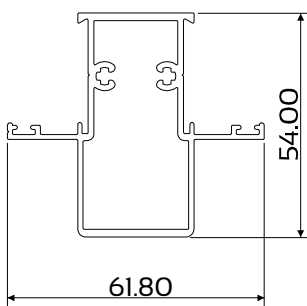
DIE No. W54651A Swift 30.5 Mullion 54mm
