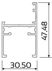
DIE No. W32028A Swift 30.5 Frame 30mm Equal Leg
