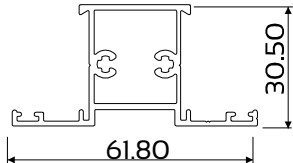
DIE No. W55685A Swift 30.5 Mullion 30mm Standard
