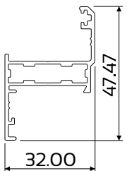
DIE No. W55441 Swift 30.5 Sash Picture Frame
