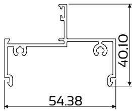
DIE No. W28481 Swift 30.5 Frame 54mm
