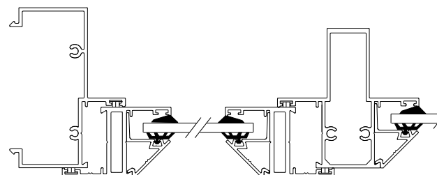
SECTION A-A Section not to scale
