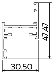
DIE No. W32027 Swift 30.5 Frame 30mm Unequal Leg
