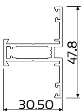
DIE No. W54867 Swift 30.5 30mm Cottage Pane Mullion
