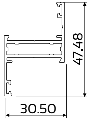
DIE No. W55684A Swift 30.5 Sash Tubular
