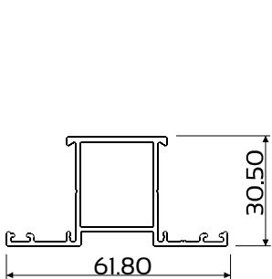
DIE No. W58308 Swift 30.5 Mullion NS
