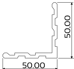
DIE No. W52695 Swift 28 Corner Cleat 50mm
