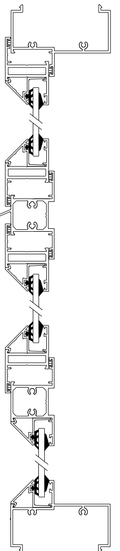
SECTION B-B Section not to scale
