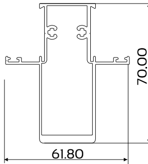
DIE No. W54652A Swift 30.5 Mullion 70mm
