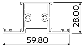
DIE No. W55683 Case 28 Mullion 28mm
