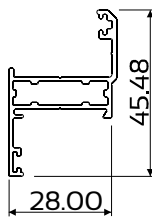
DIE No. W55497 Case 28 Picture Frame Sash
