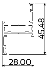
DIE No. W55682 Case 28 Sash Tubular
