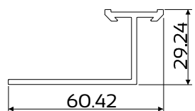
DIE No. W24052 Case 28 Fixing Lug Twist In
