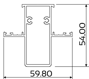
DIE No. W54348 Case 28 Mullion 54mm
