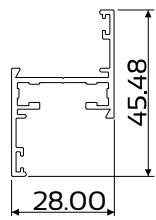
DIE No. W32025 Case 28 Frame 28mm Unequal Leg
