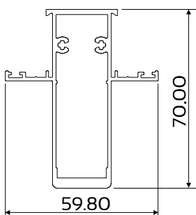
DIE No. W54329 Case 28 Mullion 70mm
