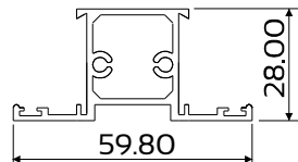
DIE No. W52697 Case 28 Mullion 28mm Standard
