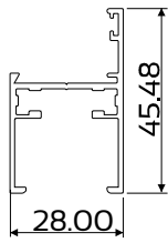
DIE No. W32026 Case 28 Frame 28mm Equal Leg
