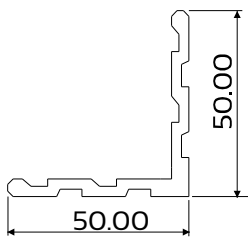
DIE No. W52695 Case 28 Corner Cleat 50mm
