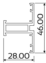
DIE No. W53283 Case 28 Mullion 28mm Cottage Pane
