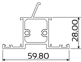
DIE No. W13142 Case 28 Mullion 28mm W/Bar
