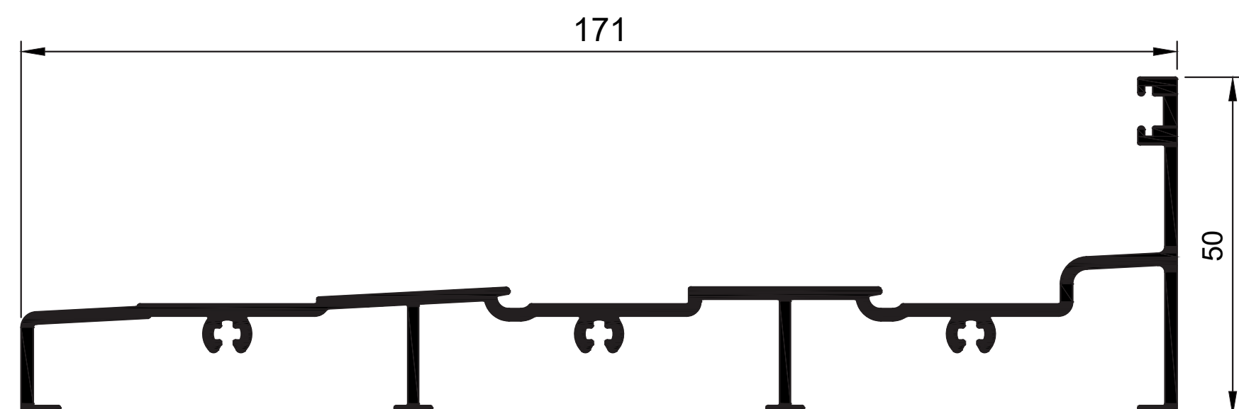
W31535 Palace M Frame Sill Rail Triple 50mm Ix = 187.697 cm 4
