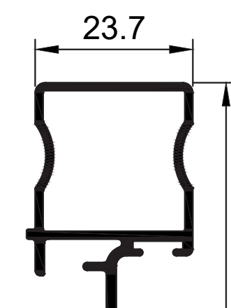
W58269 Palace M Astragal 88mm Ix = 26.741 cm 4
