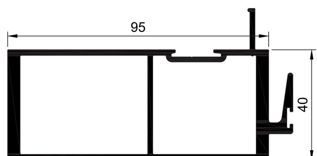
W55370 Palace M Interlock Slide 40mm HD Ix = 118.258 cm 4
