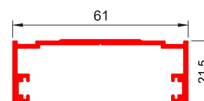
W37989 Palace M Adaptor Frame Jamb 20mm Deep
