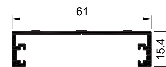
W31590 Palace M Adaptor Frame Jamb 14mm Deep
