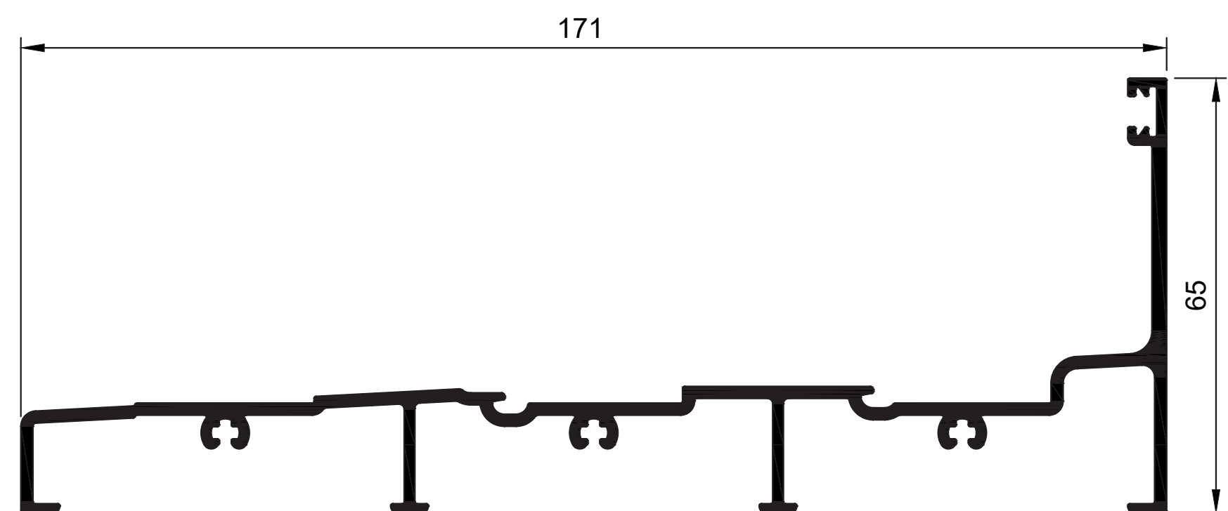
W37991 Palace M Frame Sill Rail Triple 65mm Ix = 204.583 cm 4
