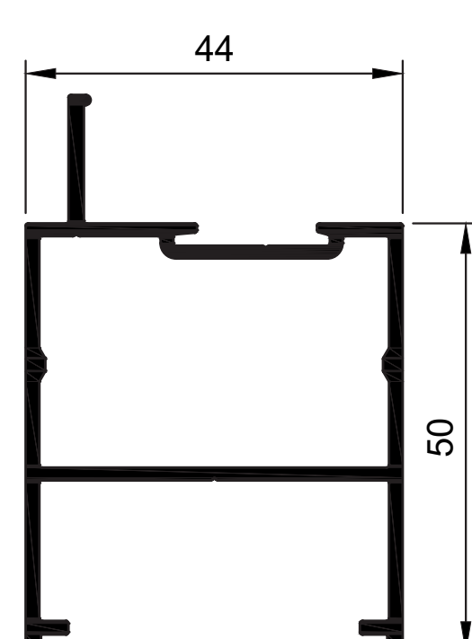
W44087 Clip 44 Head/Sill Rail 50mm R7 Ix = 10.233 cm 4
