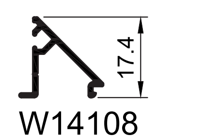
W14108 Clip 44 Bead Bevel Std
