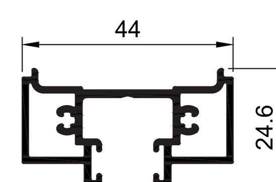
W58916 Palace M Adaptor Multi Sill Rail
