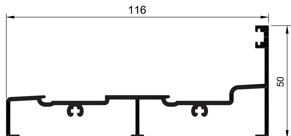
W31539 Palace M Frame Sill Rail Double 50mm Ix = 67.619 cm 4
