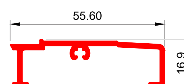
W38184 Palace M Frame Sill Rail Add On Ix = 6.491 cm 4
