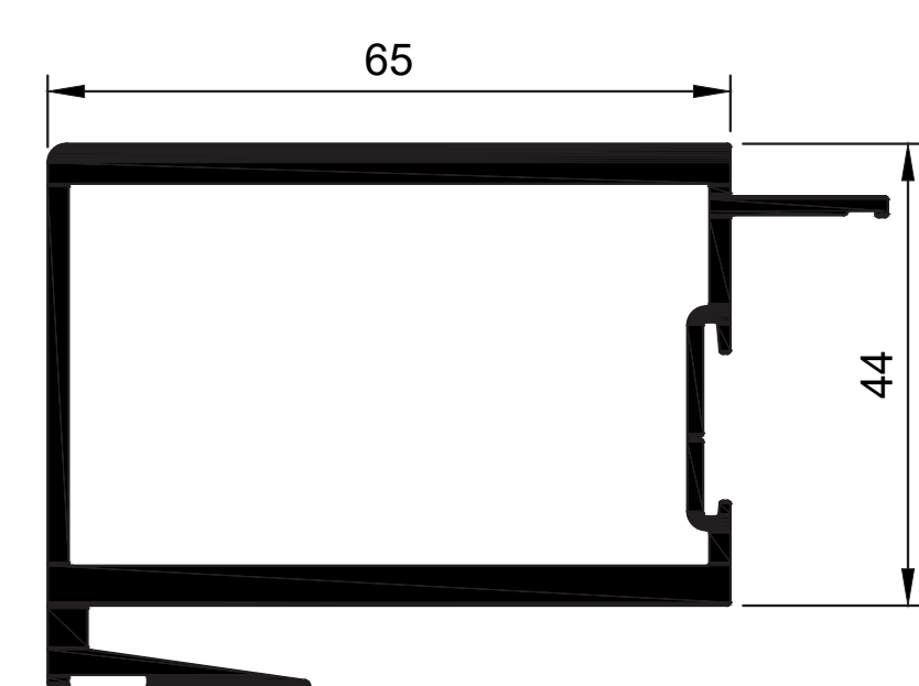
W56206 Palace M Interlock Fixed 65mm Ix = 8.028 cm 4
