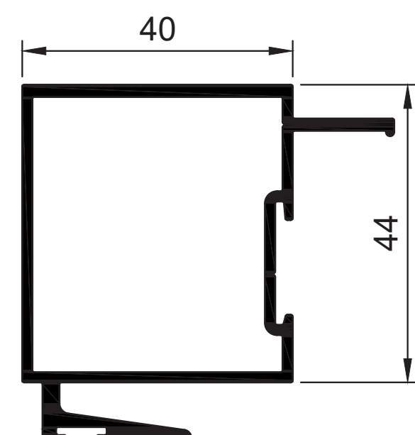
W53098 Palace M Interlock Fixed 40mm Ix = 13.343 cm 4
