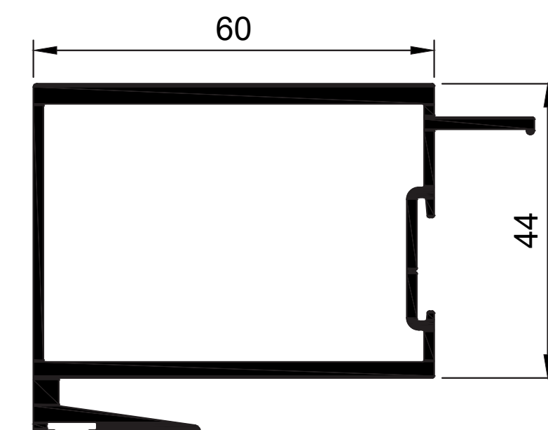
W57971 Palace M Interlock Fixed 60mm Ix = 22.511 cm 4
