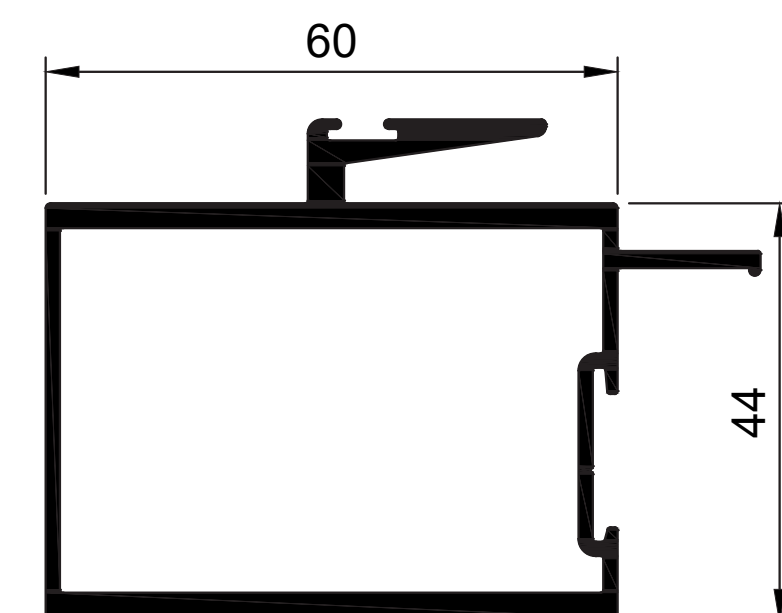
W57972 Palace M Interlock Slide 60mm Ix = 22.701 cm 4
