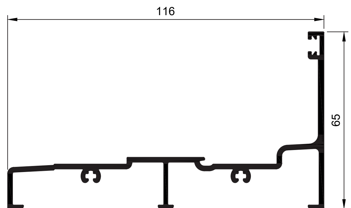
W37992 Palace M Frame Sill Rail Double 65mm Ix = 73.530 cm 4
