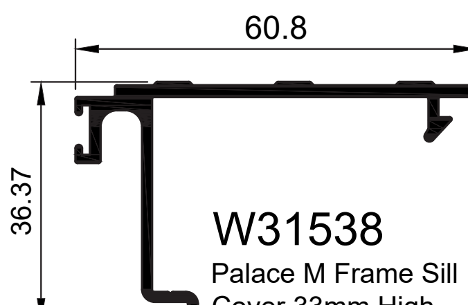
W31538 Palace M Frame Sill Cover 33mm High
