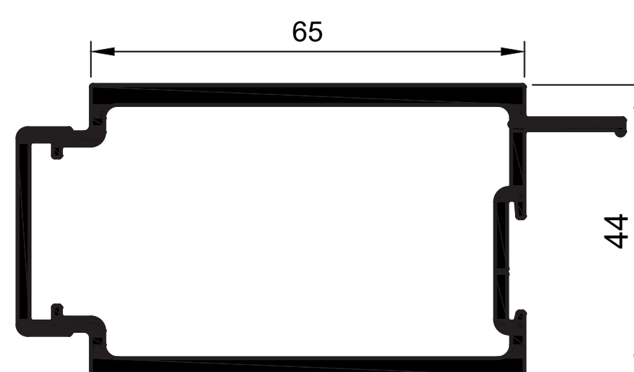
W56607 Palace M Stile Meeting 65mm Ix = 20.143 cm 4
