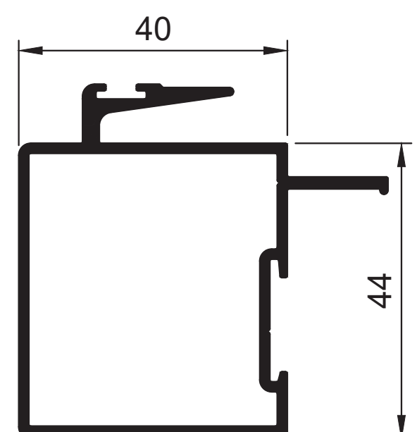
W53101 Palace M Interlock Slide 40mm Ix = 12.523 cm 4
