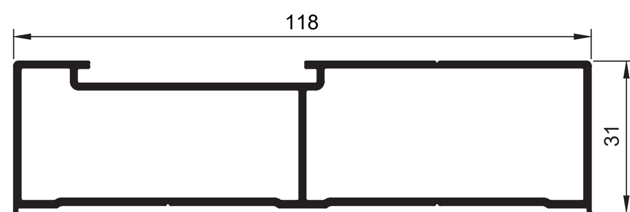
W55433 Palace M Frame Jamb Double Ix = 69.708 cm 4
