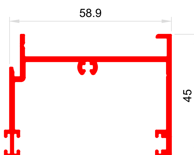
W38183 Palace M Frame Head Rail Add On Ix = 17.703 cm 4
