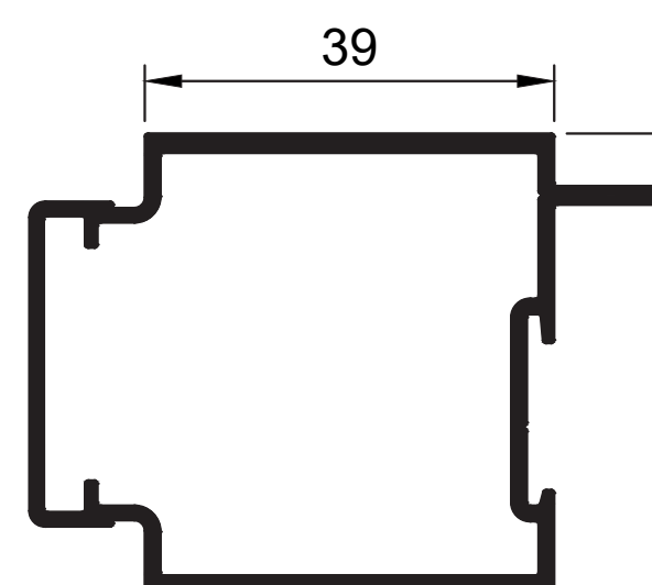
W53100 Palace M Stile Meeting 39mm Ix = 9.584 cm 4
