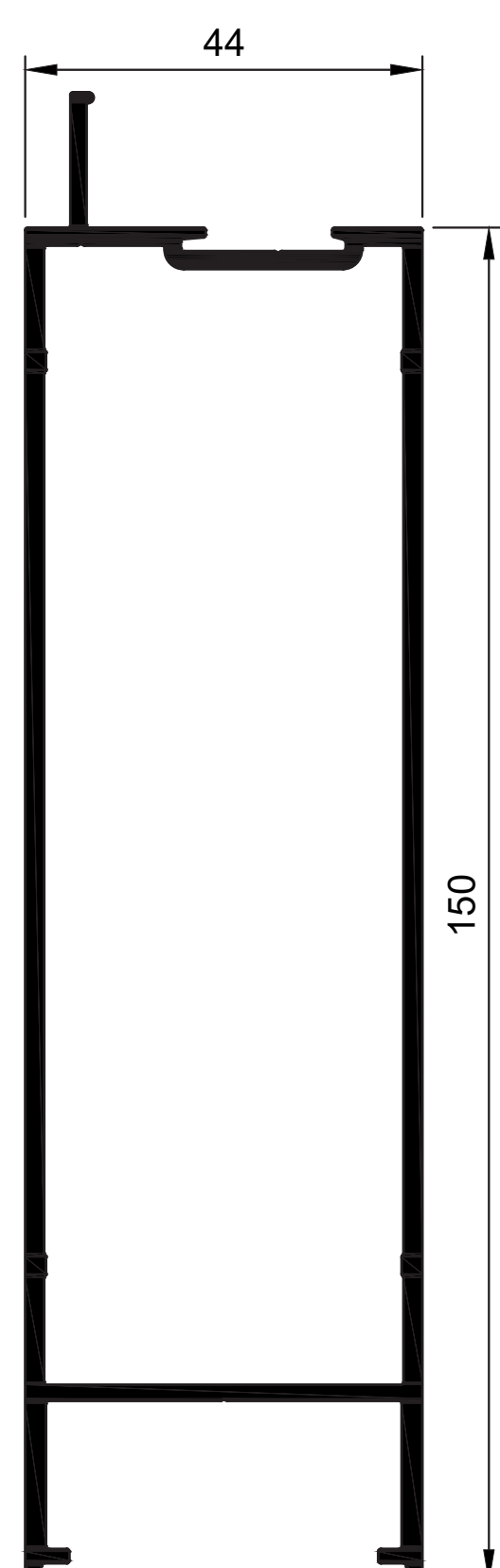
W44094 Clip 44 Head/Sill Rail 150mm R6 Ix = 31.081 cm 4
