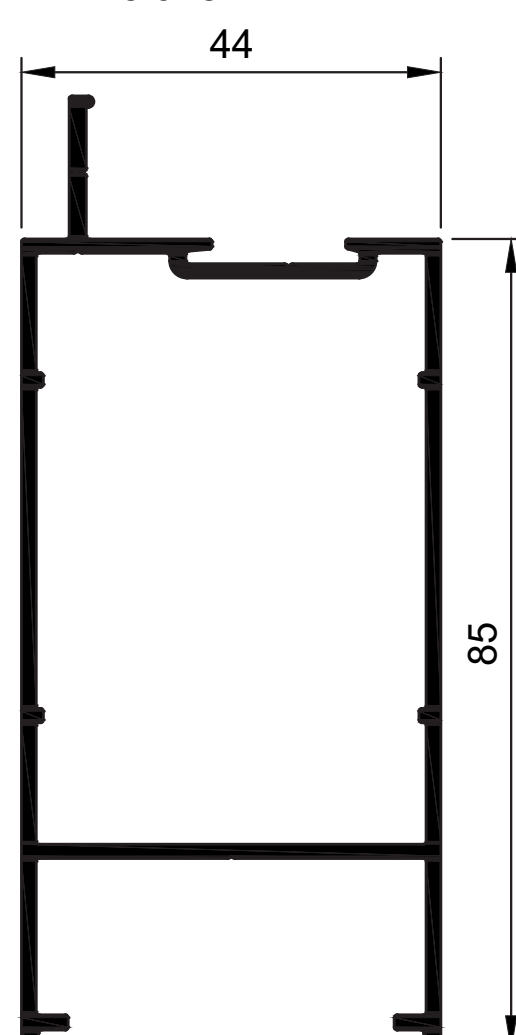
W44088 Clip 44 Head/Sill Rail 85mm R4 SD Ix = 15.019 cm 4
