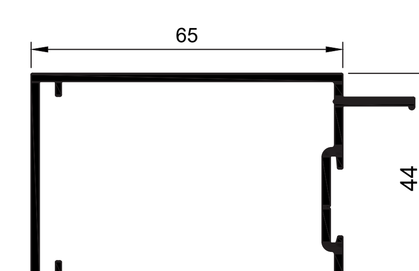
W55859 Clip44 Stile 65mm Ix = 12.855 cm 4
