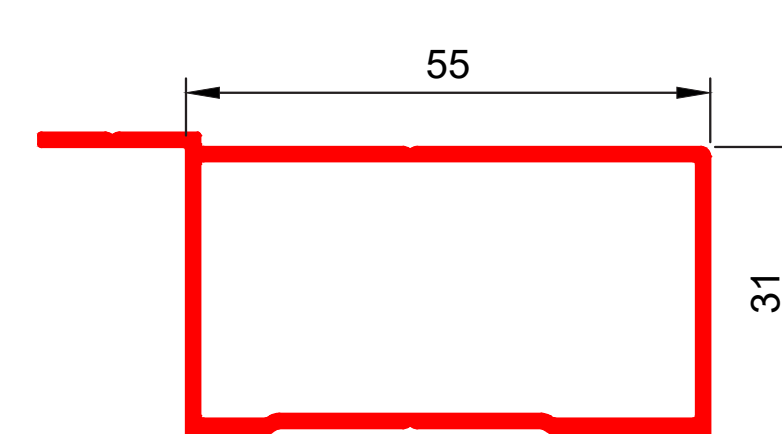
W59254 Palace M Frame Jamb Add On Ix = 12.856 cm 4
