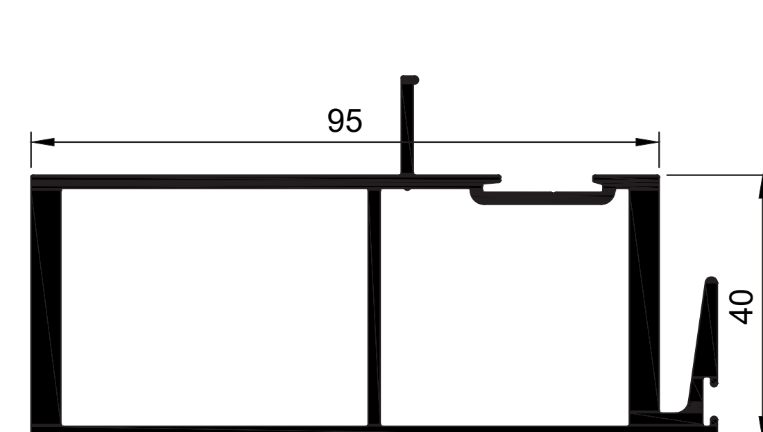
W55371 Palace M Interlock Fixed 40mm HD Ix = 117.519 cm 4
