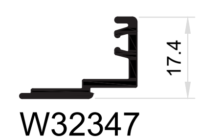
W32347 Clip 44 Bead Double Glazing 33mm
