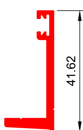
W37993 Palace M Adaptor Frame Panel Retention
