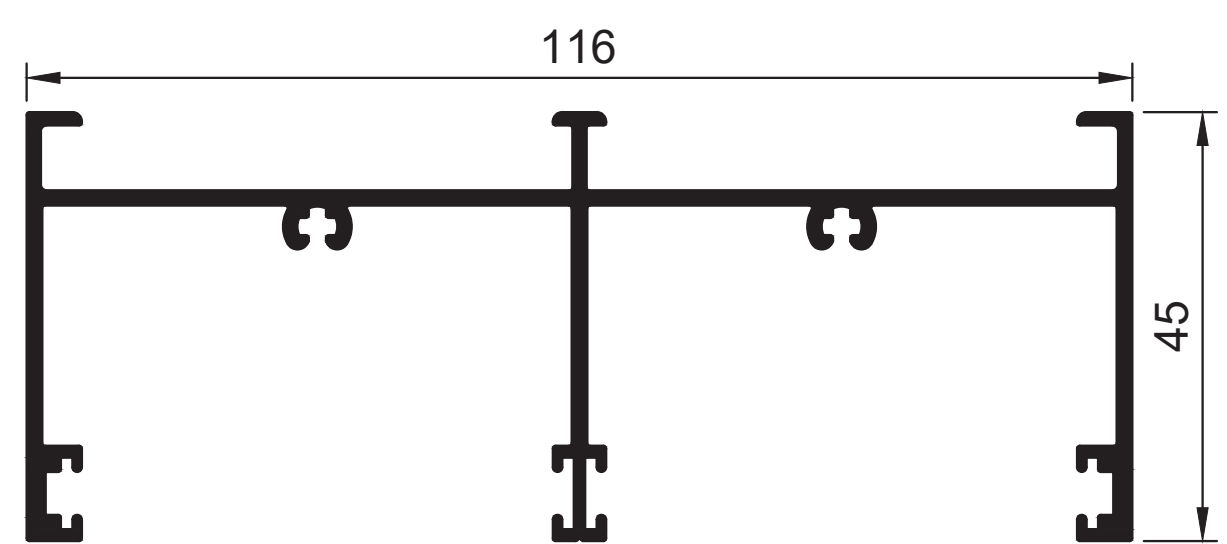
W31533 Palace M Frame Head Rail Double Ix = 85.330 cm 4
