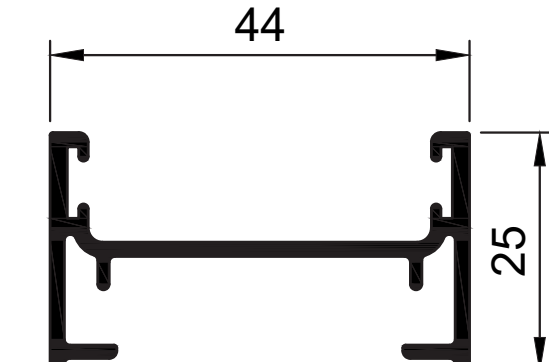
W26399 Palace M Astragal
