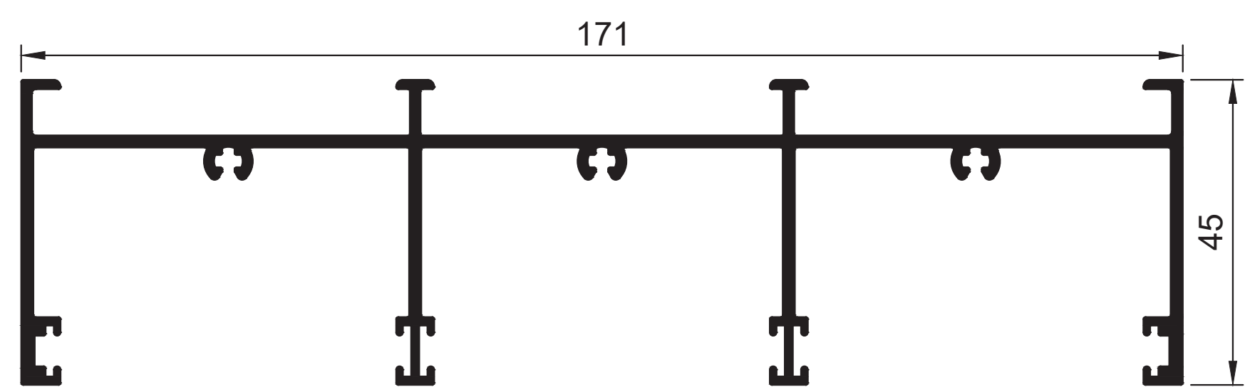
W31537 Palace M Frame Head Rail Triple Ix = 241.972 cm 4
