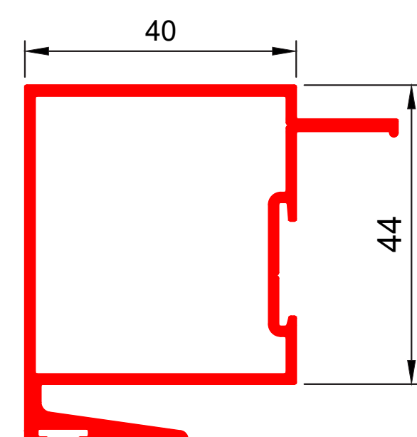
W59149 Palace M Interlock Fixed 40mm (New) Ix = 13.549 cm 4
