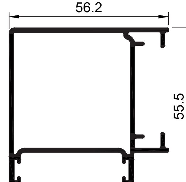
W55383 Astragal Corner Entry Vist/Pal Ix = 14.692 cm 4
