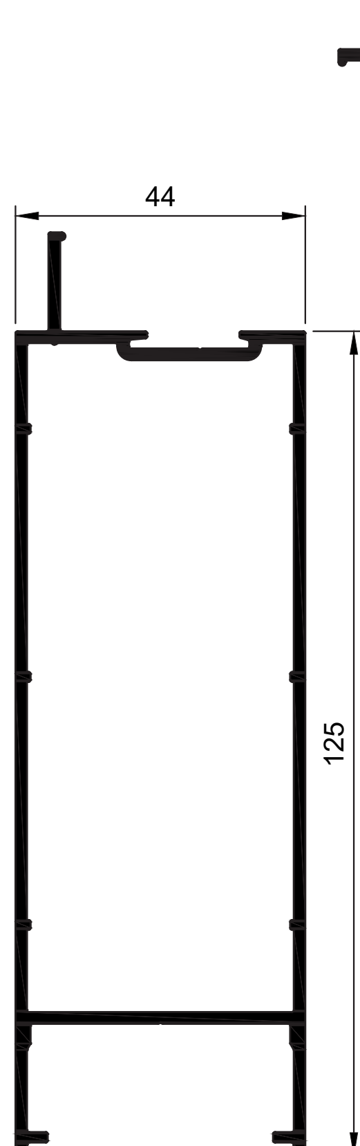
W55914 Clip 44 Head/Sill Rail 125mm R5 Ix = 23.048 cm 4
