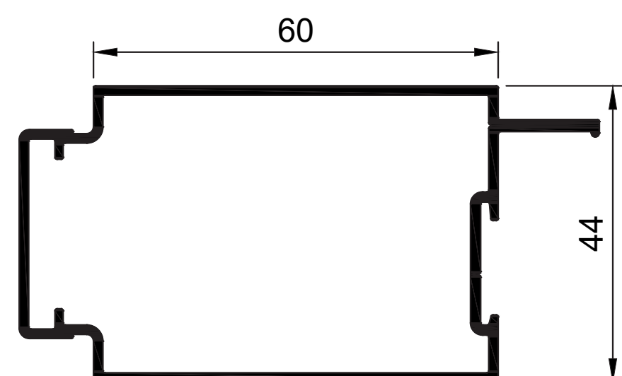
W58268 Palace M Stile Meeting 60mm Ix = 10.829 cm 4
