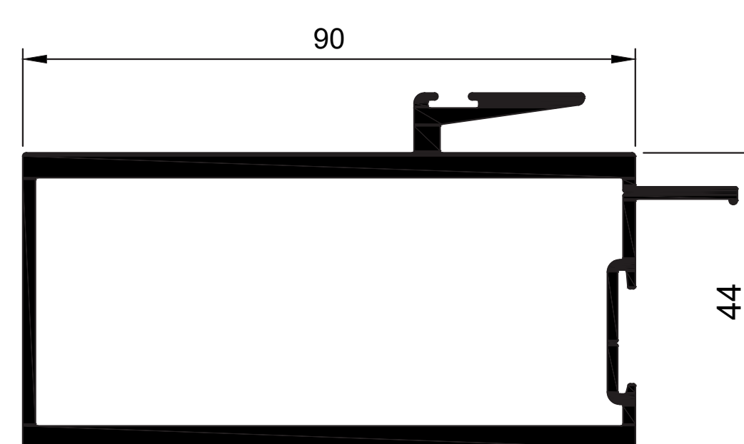
W54964 Palace M Interlock Slide 90mm Ix = 35.521 cm 4
