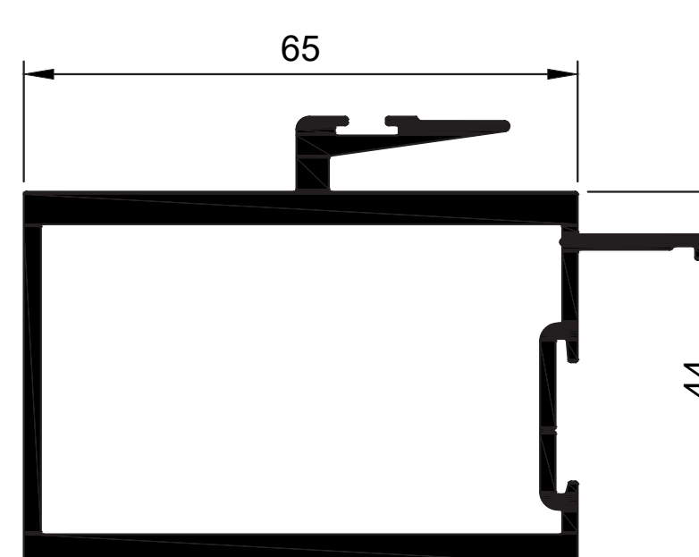
W56205 Palace M Interlock Slide 65mm Ix = 27.689 cm 4
