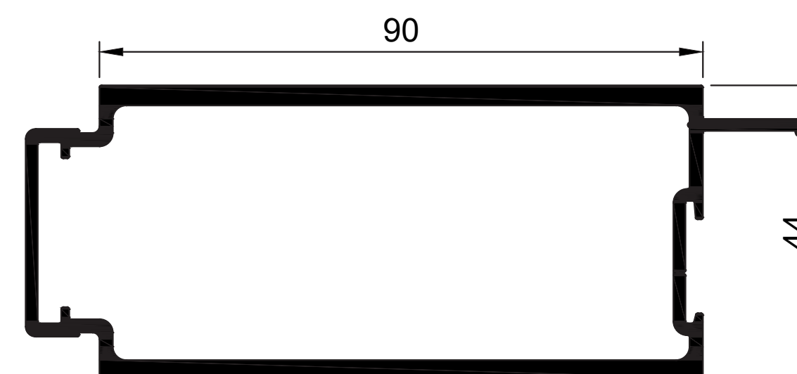
W54966 Palace M Stile Meeting 90mm Ix = 26.464 cm 4
