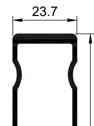
W53223 Palace M Astragal Heavy Duty Ix = 85.325 cm 4
