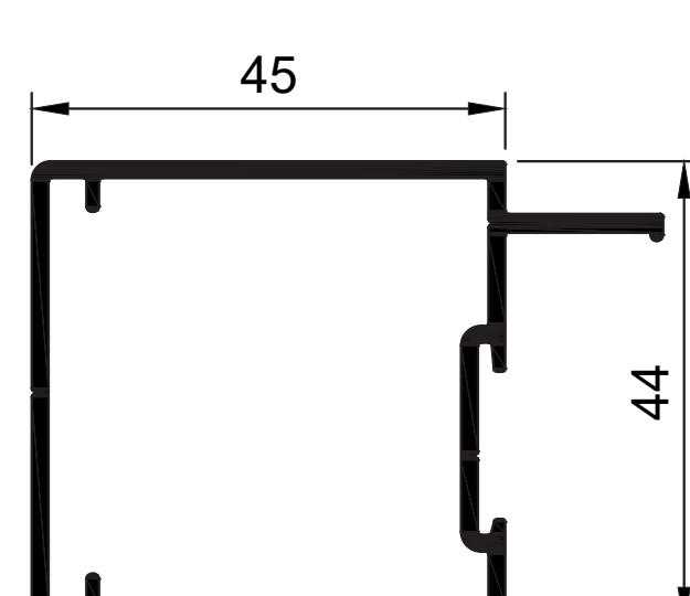
W44085 Clip44 Stile 45mm R1 SD Ix = 9.272 cm 4
