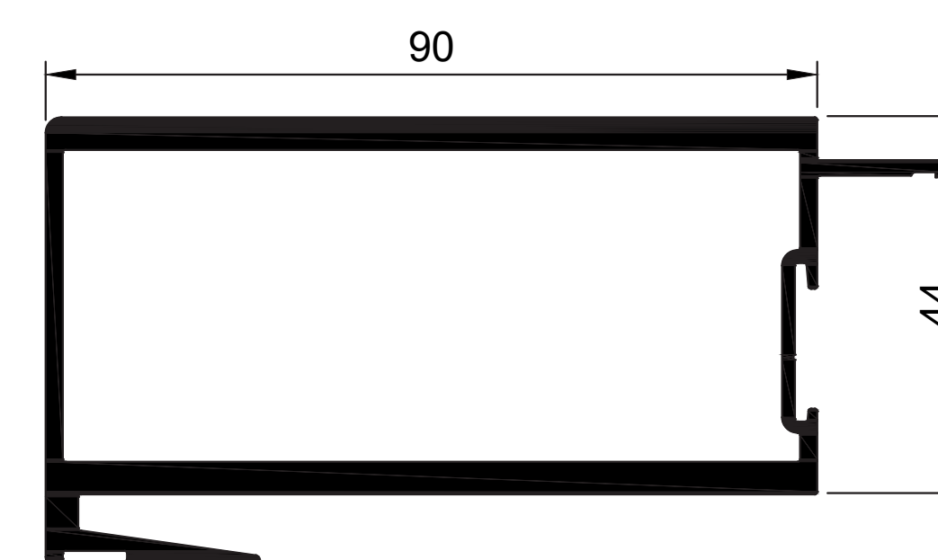
W54965 Palace M Interlock Fixed 90mm Ix = 35.814 cm 4
