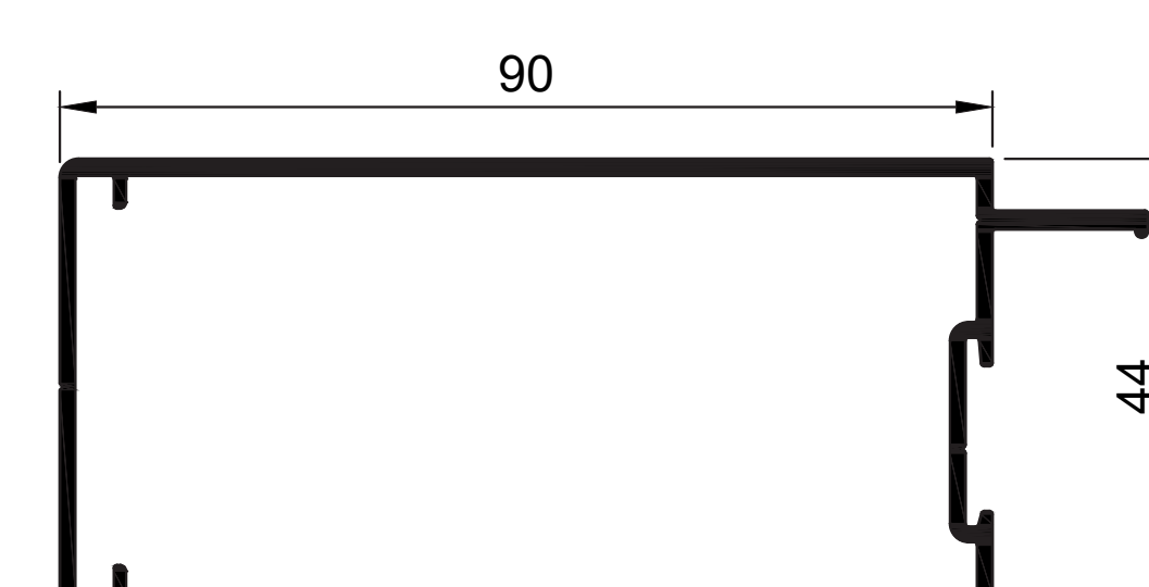
W53406 Clip44 Stile 90mm R9 SD Ix = 16.001 cm 4
