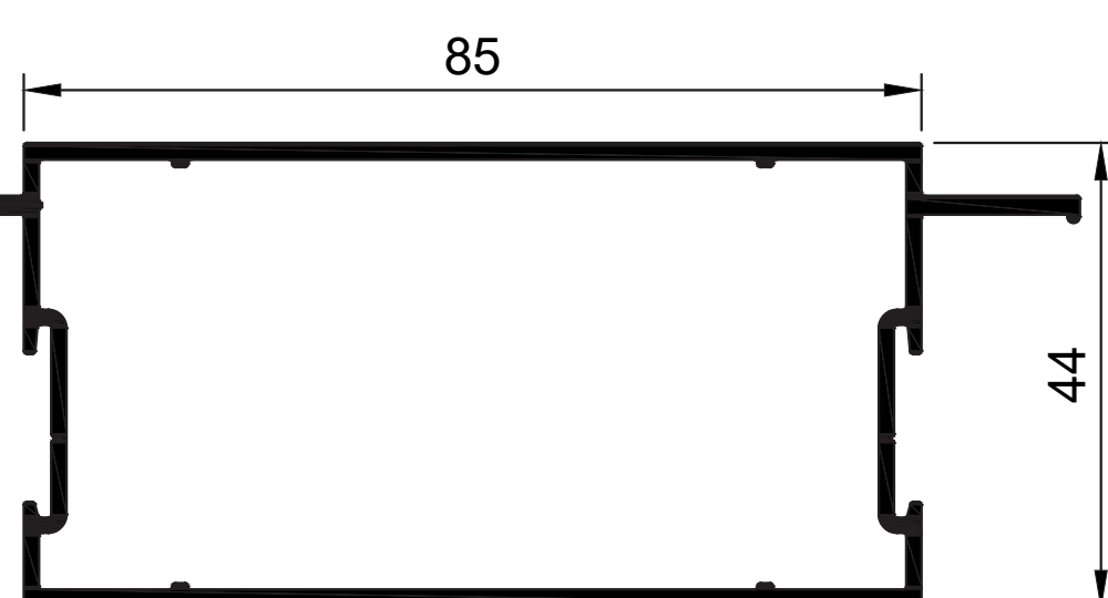
W44089 Clip44 Mid rail 85mm R4 SP Ix = 15.928 cm 4
