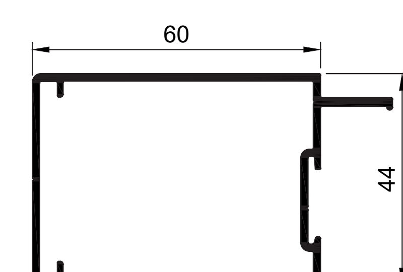
W53099 Clip44 Stile 60mm R11 SD Ix = 11.104 cm 4
