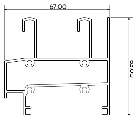
DIE No. W55169 Elite Frame Sill
