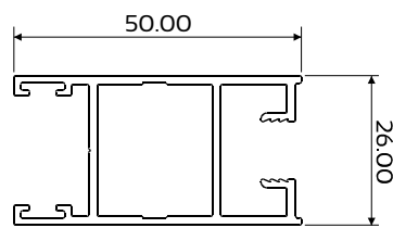
DIE No. W55166 Elite Lock Stile
