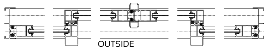
SECTION A-A Section not to scale
