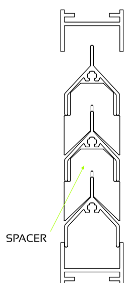
SECTION B-B Section not to scale
