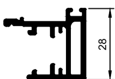
W57643 F60 Flush Glaze Frame
