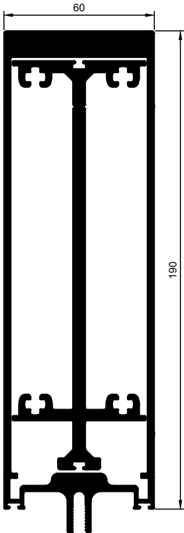
W58460 F60 Mullion Non-Thermal 190mm Ix = 1000.93 cm 4 W35361 F60 Expansion Profile 190mm Ix = 453.85 cm 4
