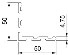
CORNER CLEAT W52695
