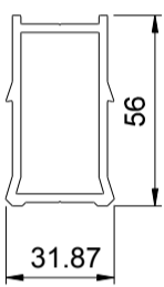
STIFFENER PROFILE W54449
